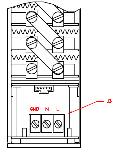
VIEW B
